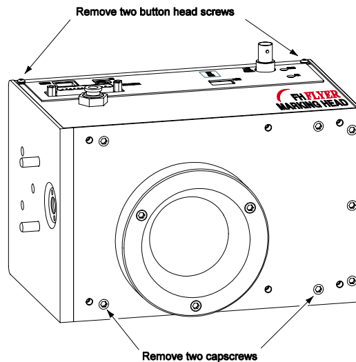
Figure 3 Opening Flyer to enable FASI
